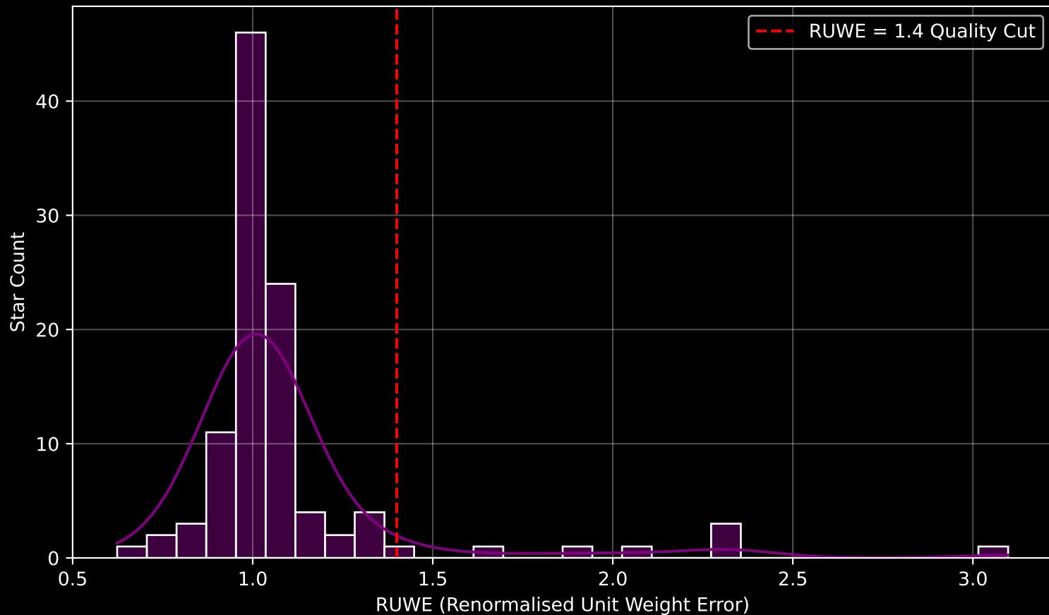
GAPOGEE DR17 Field [LMC14] RUWE Distribution (n= 105)
