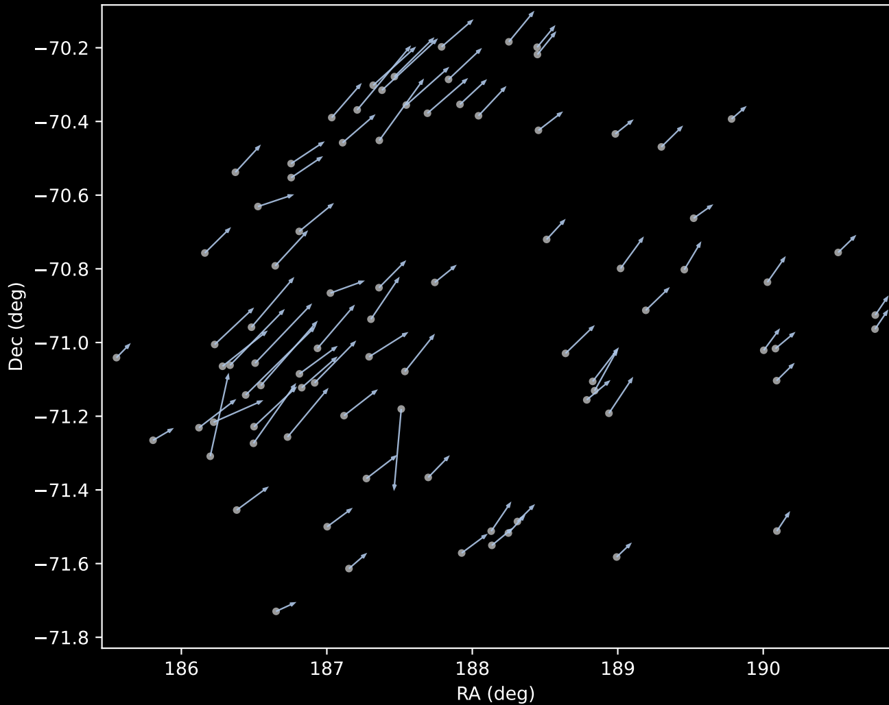
APOGEE DR17 Cluster 1 Proper Motion Vectors (n=84)
