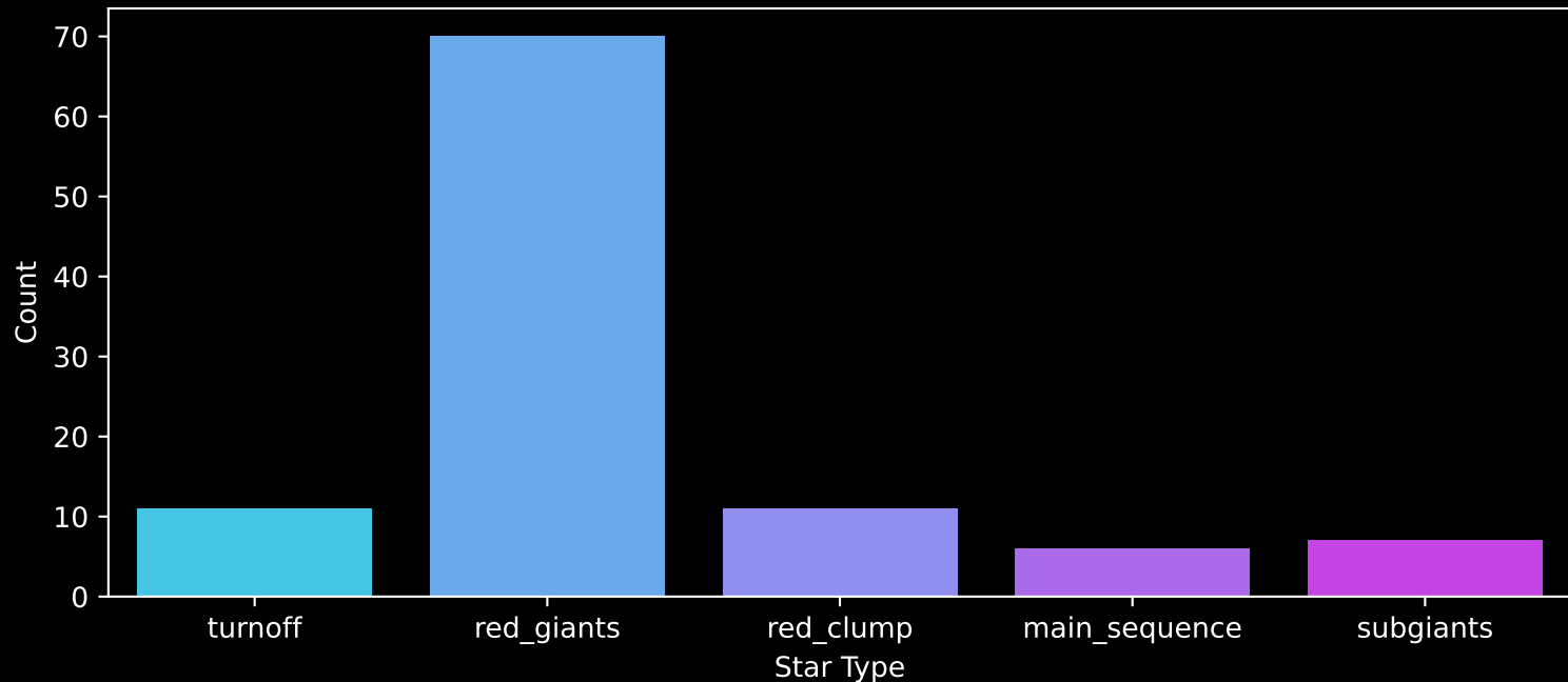
APOGEE DR17 Field: [LMC14] Count plot of Star Type
