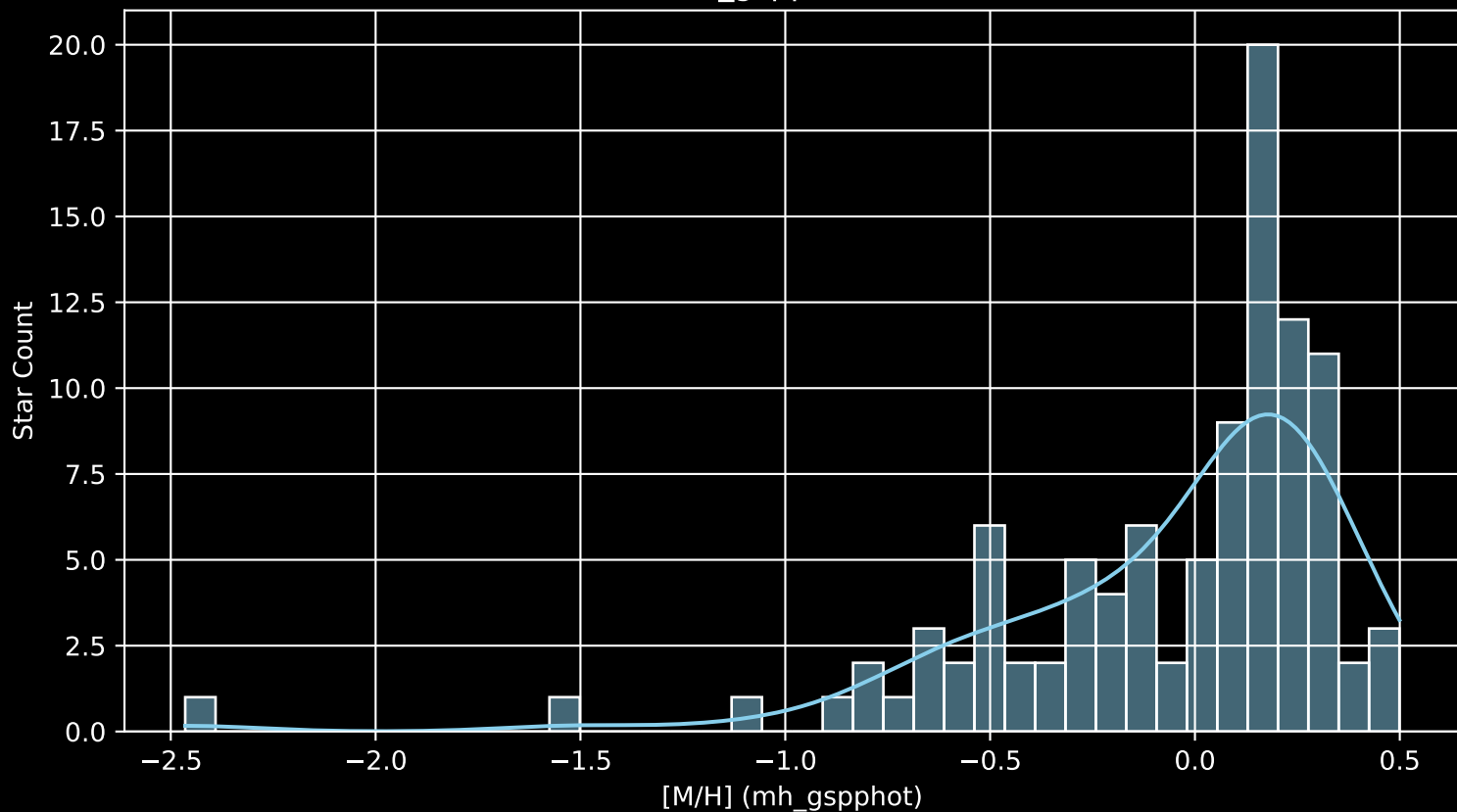
APOGEE DR17 Field: [LMC14 [M/H] (mh_gspphot) (n= 101)
