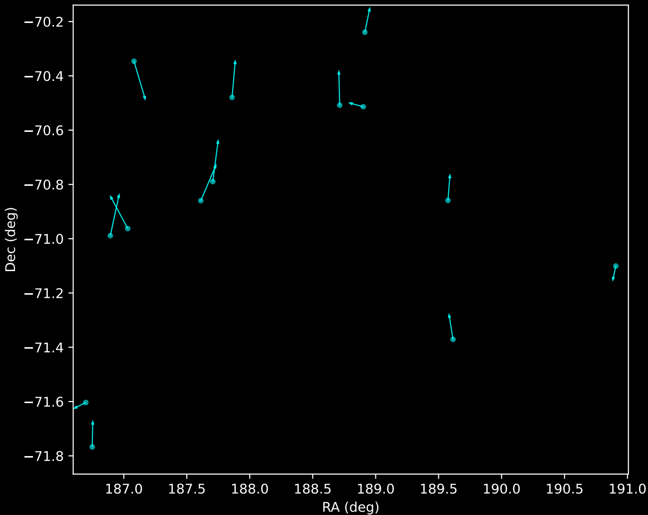
APOGEE DR17 Noise Stream Proper Motion Vectors (n=14)
