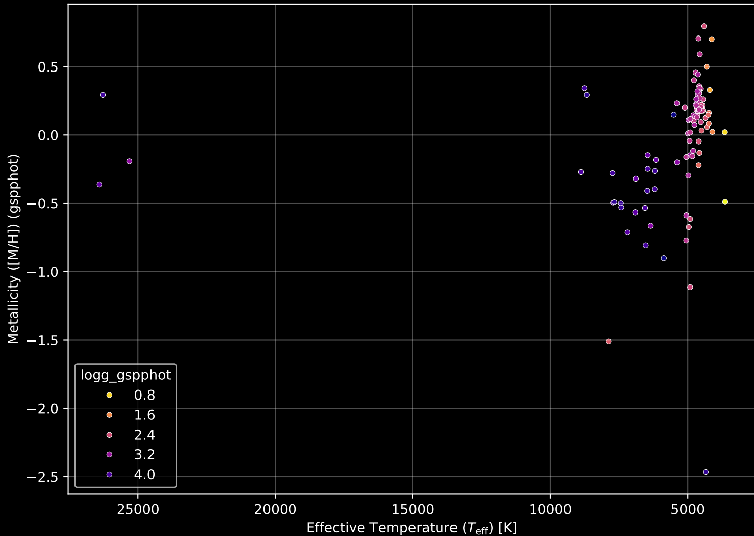
APOGEE DR17 Field: [LMC14] Stellar Population Parameters (n= 105)
