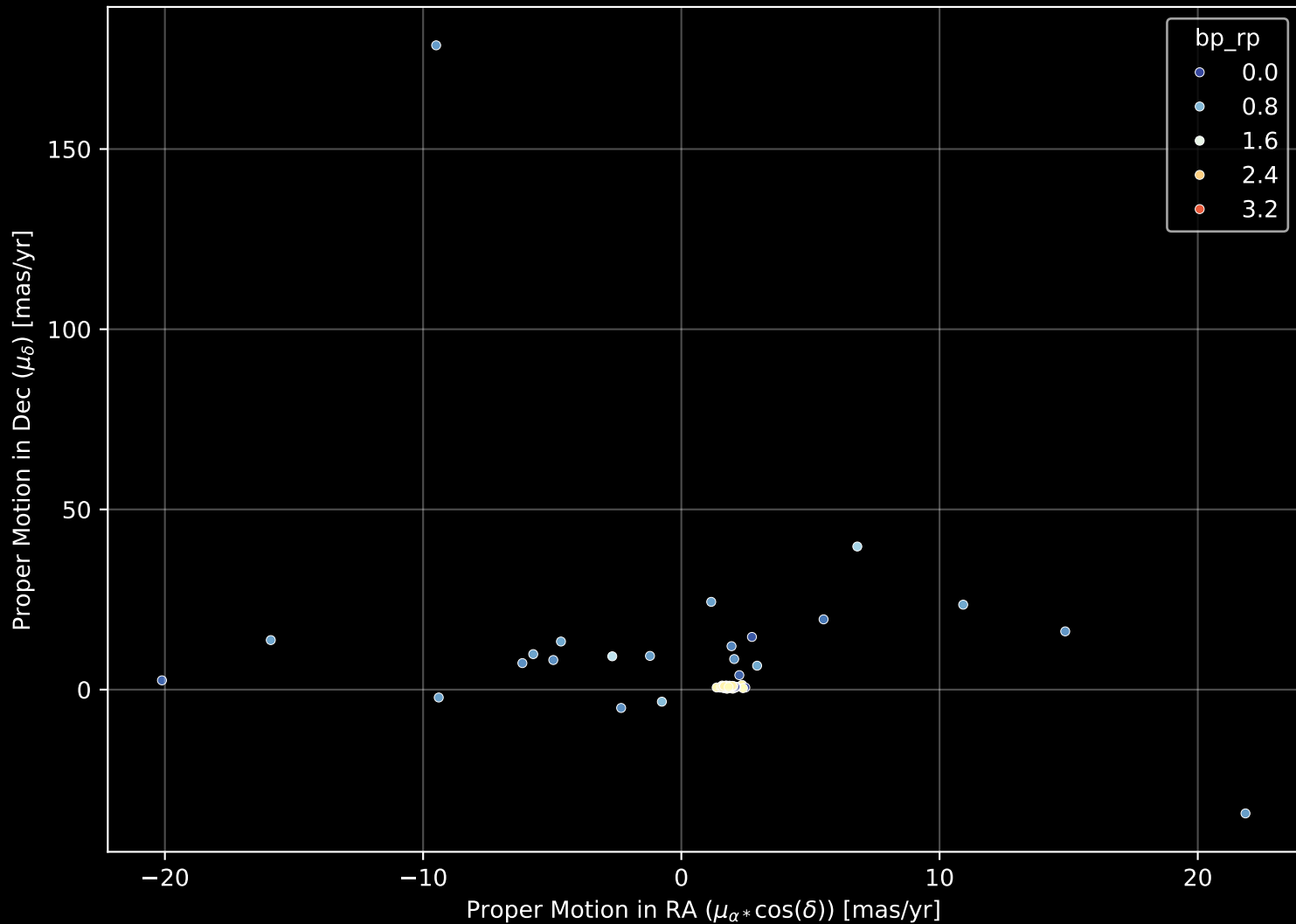
APOGEE DR17 Field: [LMC14] Proper Motion Diagram (n= 105)
