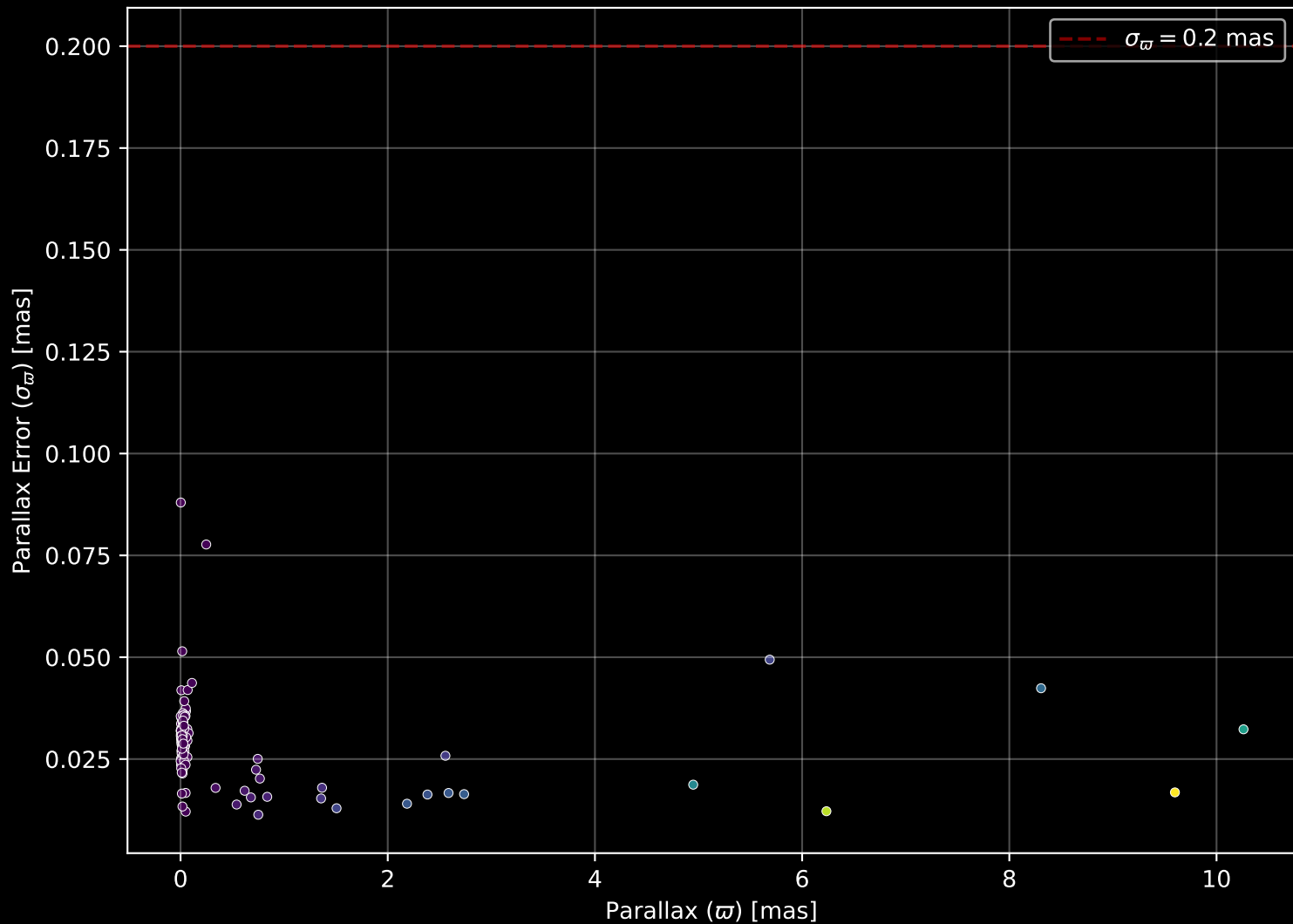
APOGEE DR17 Field: [LMC14] Parallax Quality (n= 105
